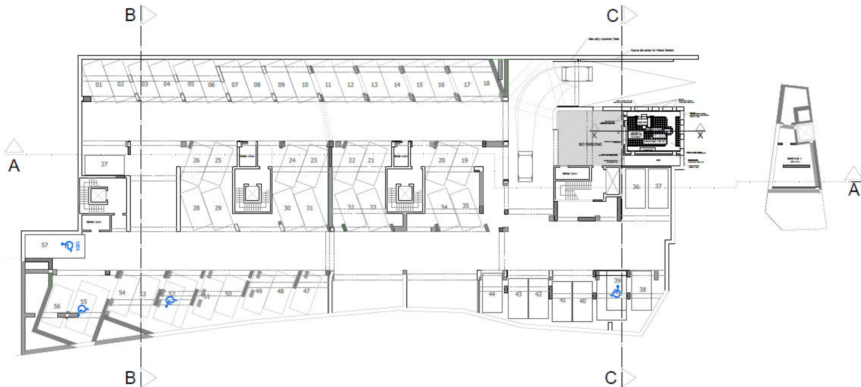
As Permitted and Proposed Basement Level Plan
